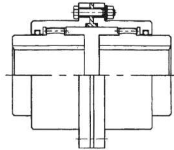
▲ INSULATION TYPE
