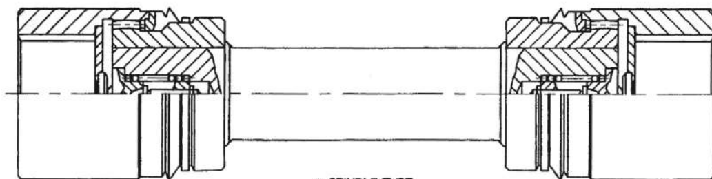
▲ SPINDLE TYPE
