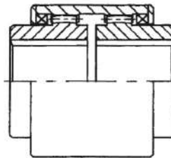
▲ SLEEVE TYPE
